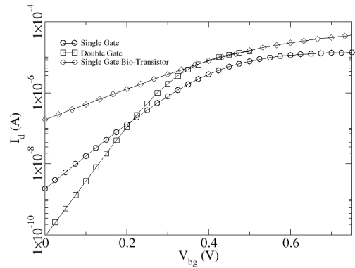
Figure 4: I_d - V_g Characteristics of the 5 nm doublegate transistor, single gate and bio-gate configurations.
