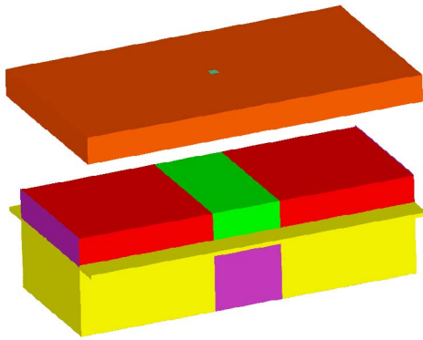
Figure 2: The Taurus simulation structure. The double gate transistor is shown at the bottom along with the lipid membrane and the small pore. Materials modelling water have been removed for clarity.
